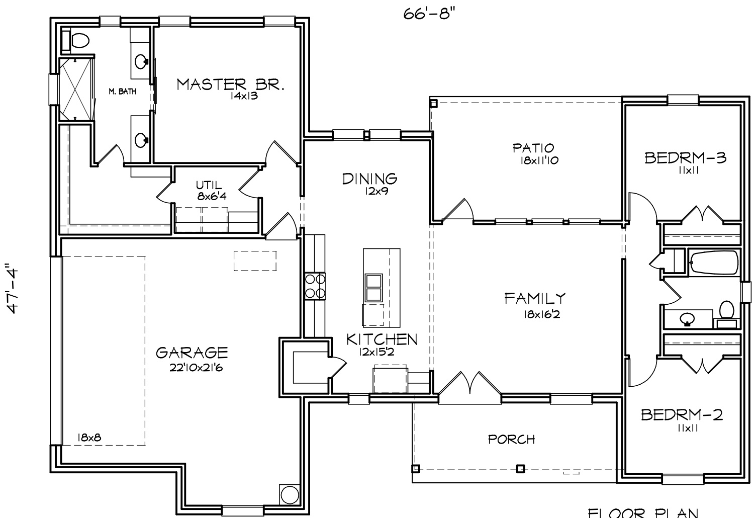
FLOOR PLAN 1612 SF
