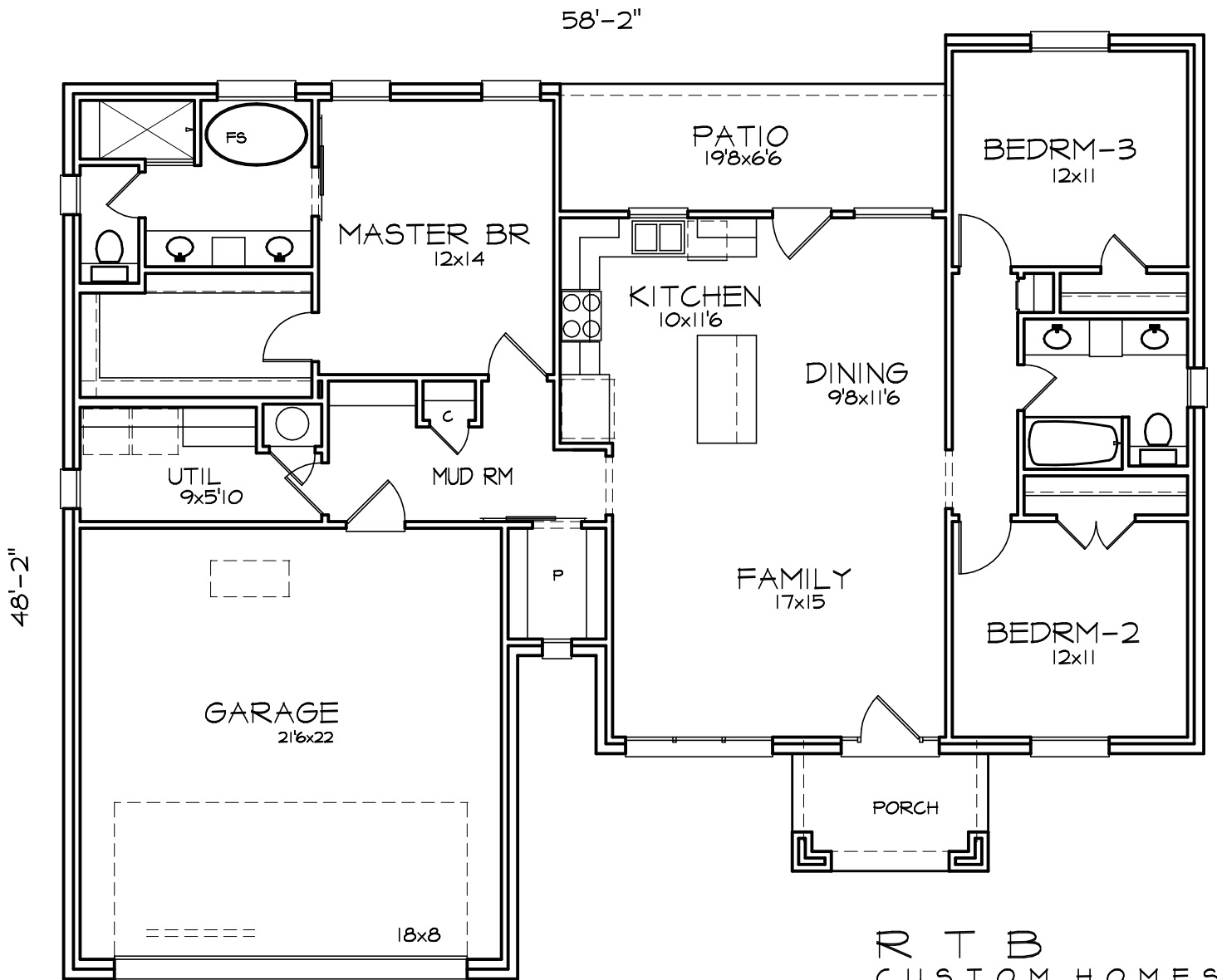
FLOOR PLAN 201231611-L 1611 SF
