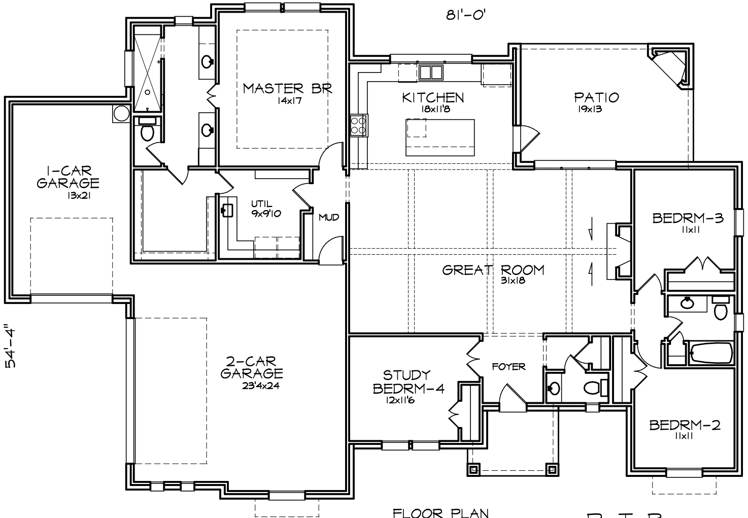
FLOOR PLAN 2238 SF
